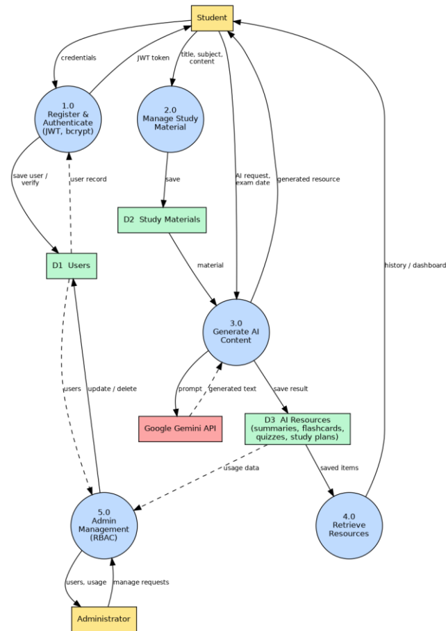
Figure 2: Level 1 DFD of AI StudyBuddy
