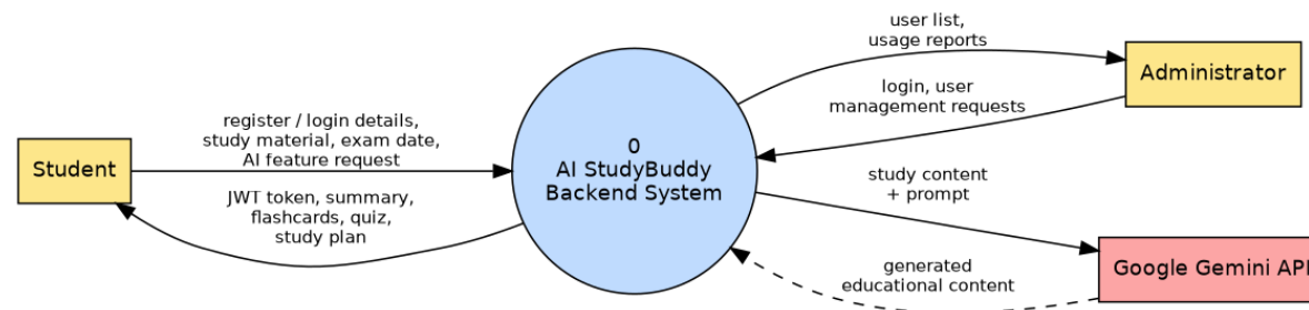
Figure 1: Level 0 DFD of AI StudyBuddy
